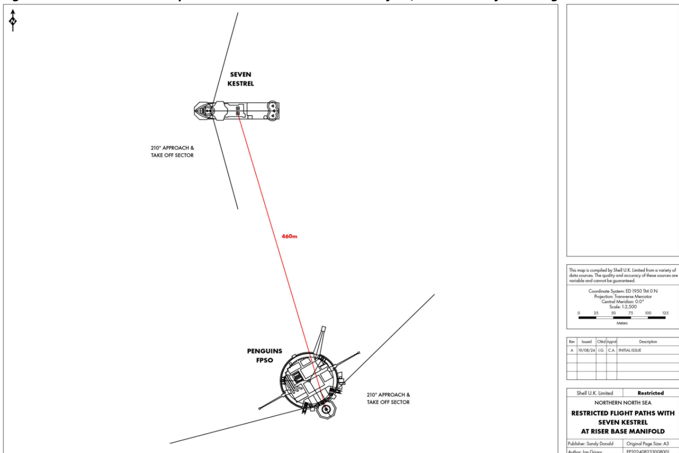
Figure 1 – The Seven Kestrel positioned at the Riser Base Manifold, Northwest of the Penguins FPSO.
