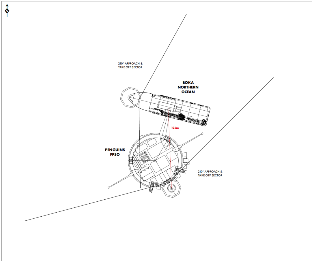
Figure 1 – Boka Northern Ocean in North-Easterly position alongside the Penguins FPSO
