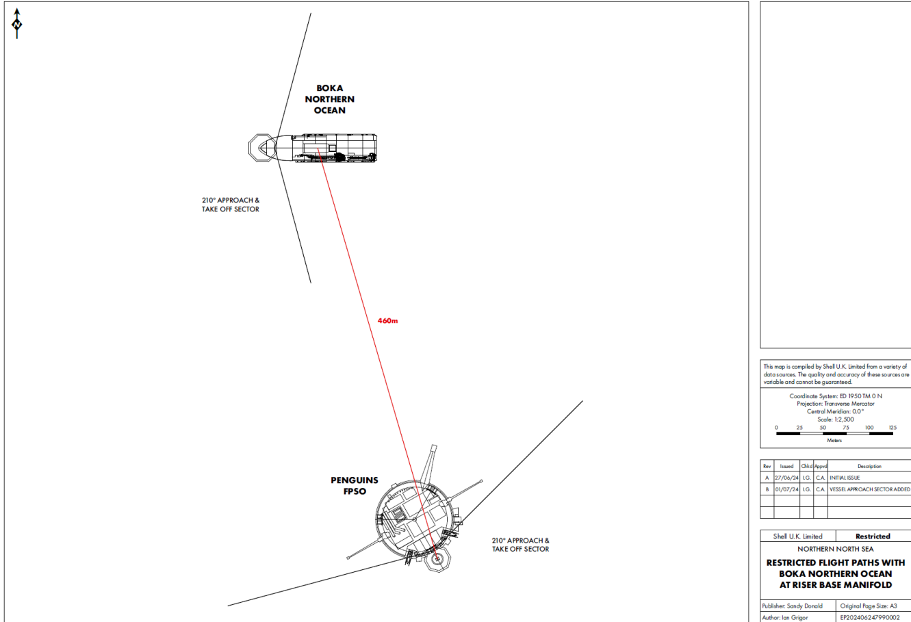
Figure 2 – The Boka Northern Ocean positioned at the Riser Base Manifold, North of the Penguins FPSO.
