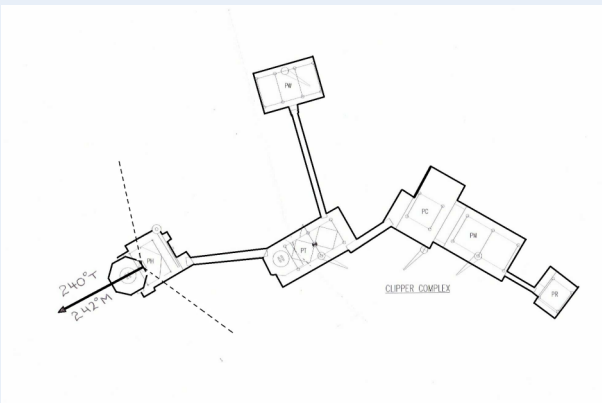
PLAN DRAWING
